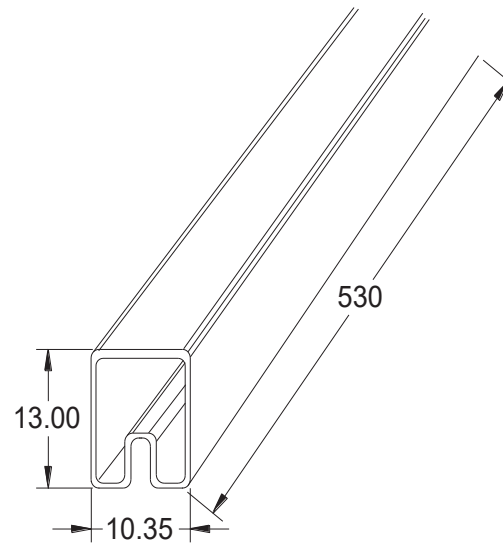
Tube: 535*13.0*10.35mm
