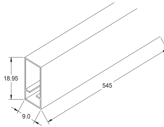
Tube: 545*9.0*18.95mm
