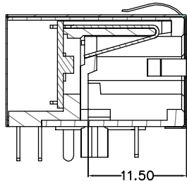
CRROSS SECTION
