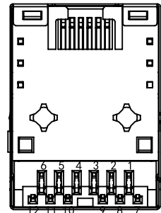
BOTTOM VIEW
