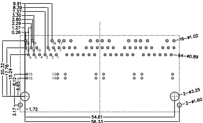
RECOMMENDED PCB LAYOUT VIEWED FROM COMPONENT SIDE
