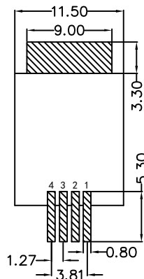
RECOMMENDED PCB LAYOUT VIEWED FROM COMPONENT SIDE
