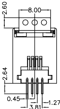
BACK VIEW
