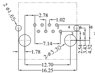
RECOMMENDED PCB LAYOUT VIEWED FROM COMPONENT SIDE
