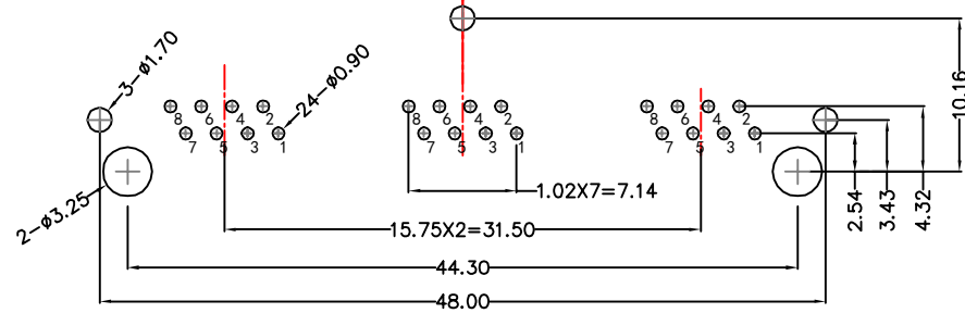
RECOMMENDED PCB LAYOUT VIEWED FROM COMPONENT SIDE
