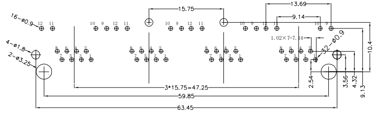
RECOMMENDED PCB LAYOUT VIEWED FROM COMPONENT SIDE
