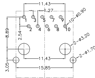
RECOMMENDED PCB LAYOUT VIEWED FROM COMPONENT SIDE
