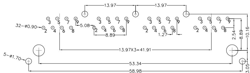
RECOMMENDED PCB LAYOUT VIEWED FROM COMPONENT SIDE
