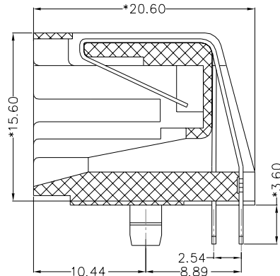
CUTAWAY VIEW
