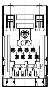
BOTTOM VIEW
