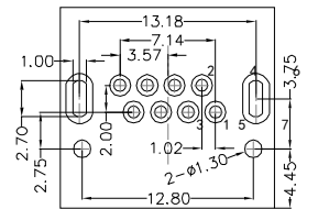
RECOMMENDED PCB LAYOUT VIEWED FROM COMPONENT SIDE
