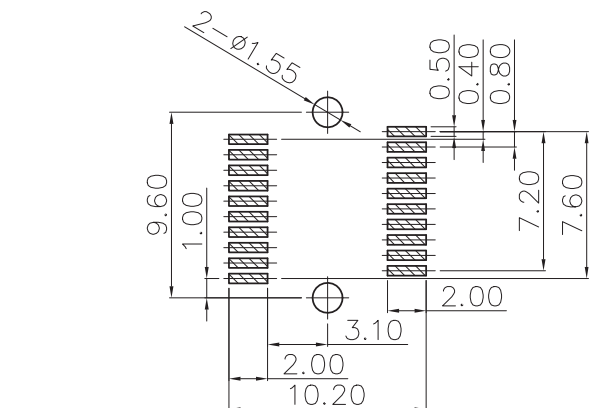
DETAIL A(SCALE 2:1)
