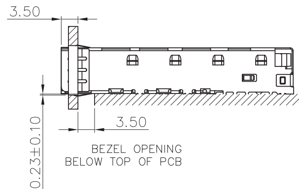
DETAIL A(SCALE 2:1)
