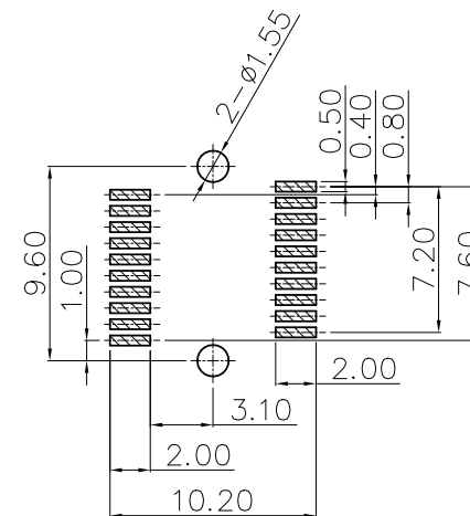
DETAIL A(SCALE 2:1)
