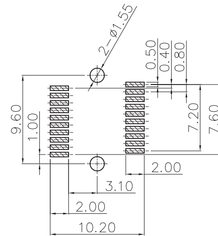
DETAIL A(SCALE 2:1)
