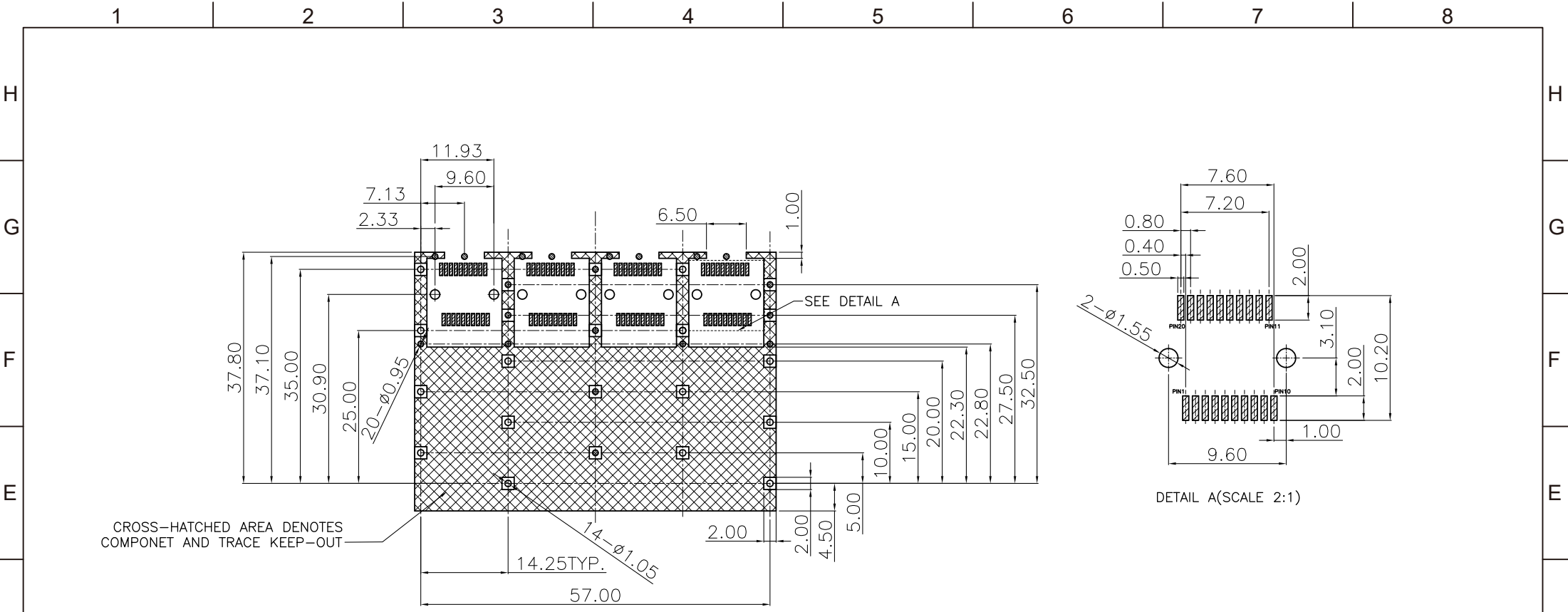
RECOMMENDED PCB LAYOUT (COMPONENT SIDE)
