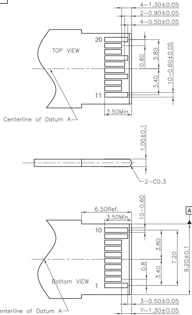
RECOMMENDED LAYOUT MATING PCB SIDE
