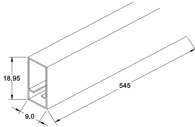
Tube: 545*9.0*18.95mm
