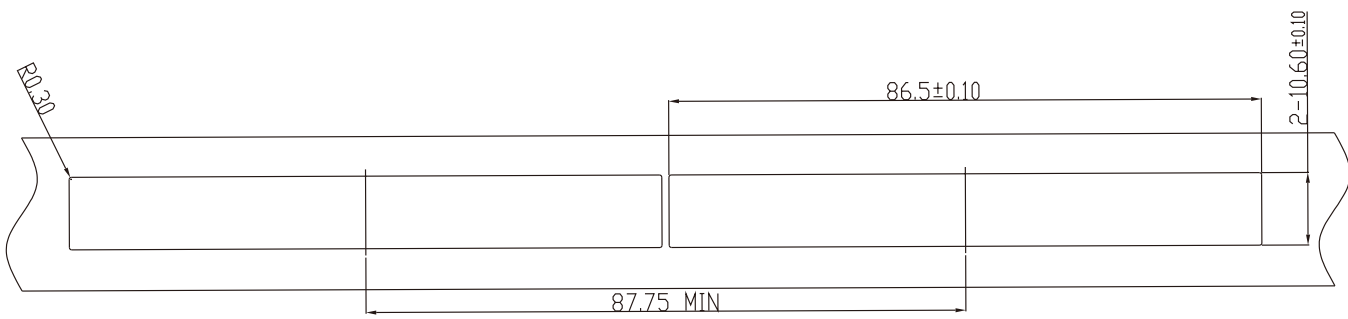
RECOMMENDED BEZEL CUT-OUT SINGLE SIDED APPLICATIONS
