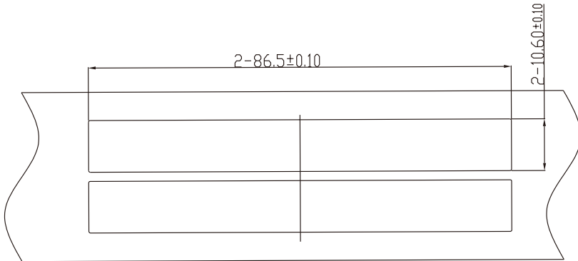
RECOMMENDED BEZEL CUT-OUT SINGLE SIDED APPLICATIONS
