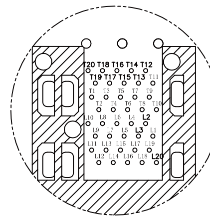
CONNECTOR PIN-OUT COMPONENT SIDE OF BOARD
