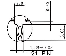
DETAIL B SCALE 5:1
