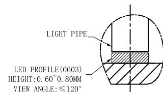
DETAIL F SCALE 4:1
