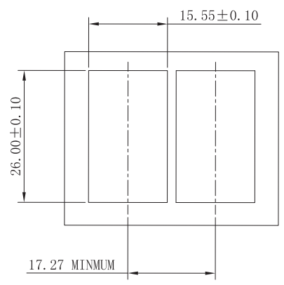
BEZEL CUT-OUT CENTER SPACING DETAIL BZZEL THICKNESS: 0.8-2.6
