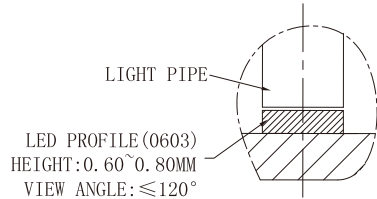
DETAILI F SCALE 4:1
