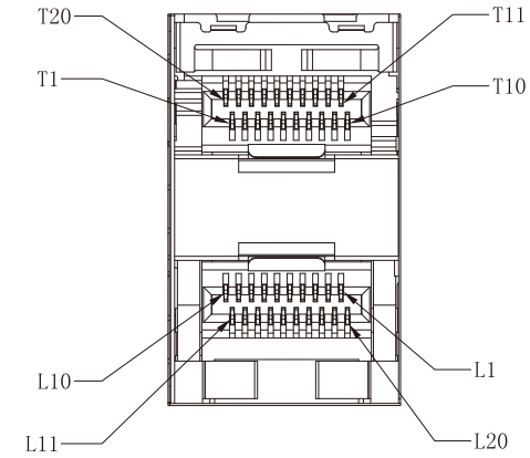
DETAIL A1 SCALE 4:1
