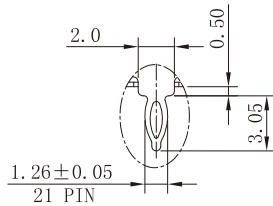
DETAIL B SCALE 5:1
