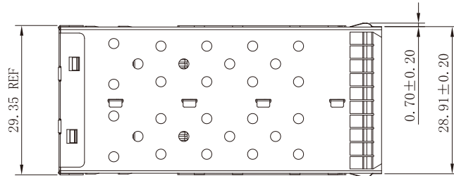
DETAIL B SCALE 5:1
