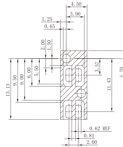
KEEPOUT ZONE DETAIL SCALE 5:1
