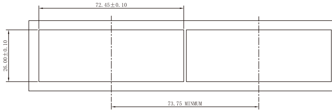
BEZEL CUT-OUT CENTER SPACING DETAIL BEZEL THICKNESS: 0.8-2.6
