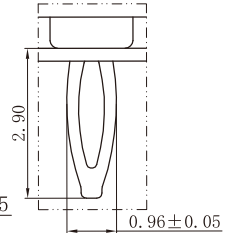
DETAIL B SCALE 10:1
