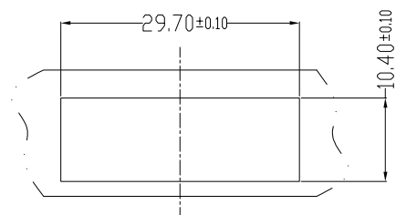
RECOMMENDED BEZEL CUT-OUT SINGLE SIDED APPLICATIONS
