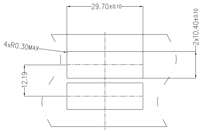
RECOMMENDED BEZEL CUT-OUT BELLY TO BELLY APPLICATIONS
