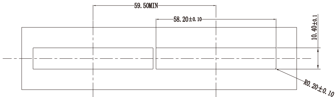
RECOMMENDED BEZEL CUT-OUT SINGLE SIDED APPLICATIONS SCALE 5:3
