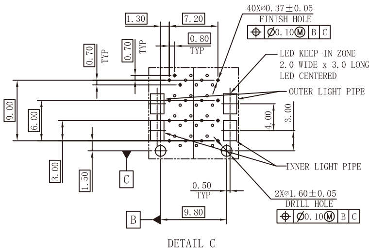
PIN MAP
