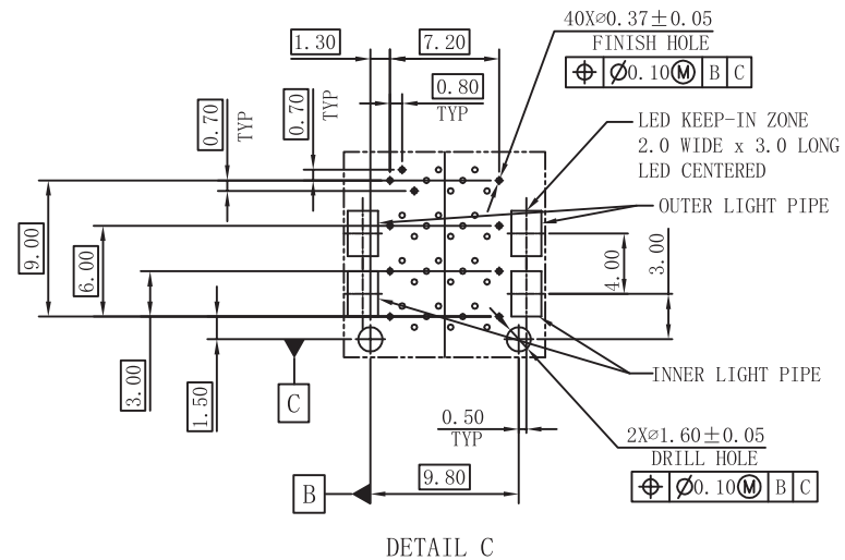
DETAIL C
