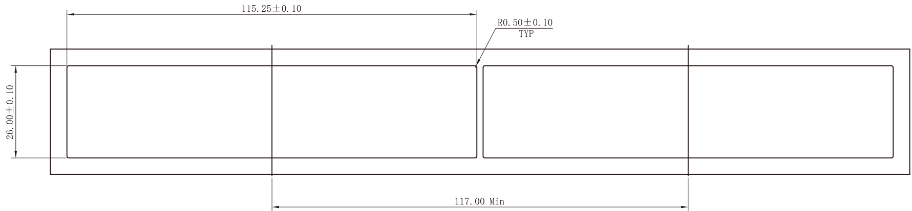
BEZEL CUT-OUT CENTER SPACING DETAIL BEZEL THICKNESS:0.8-2.6
