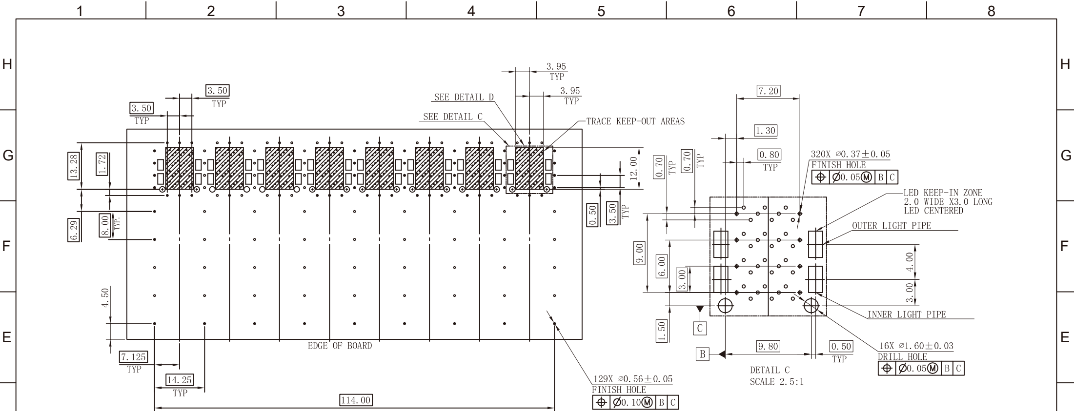
RECOMMENDED PCB LAYOUT—COMPONENT SIDE RECOMMENDED PCB THICKNESS—2.63mm
