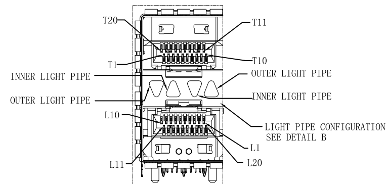
DETAIL A SCALE 2:1
