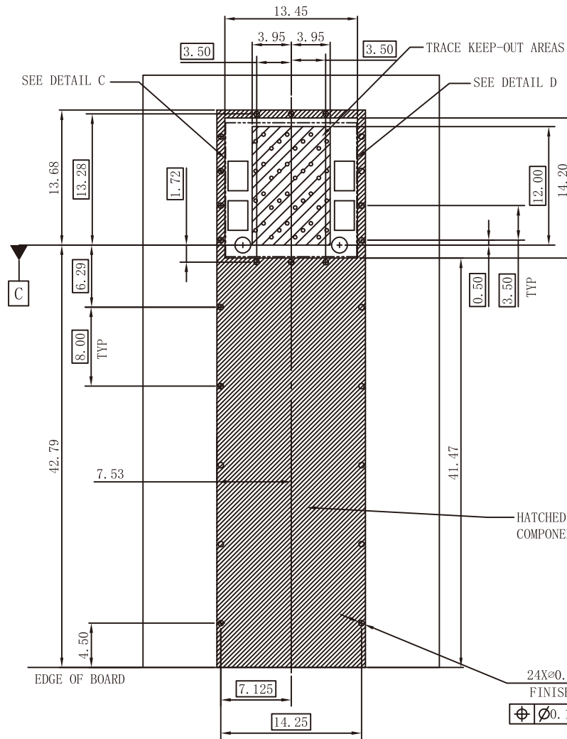
RECOMMENDED PCB LAYOUT-COMPONENT SIDE RECOMMENDED PCB THICKNESS-2.63mm
