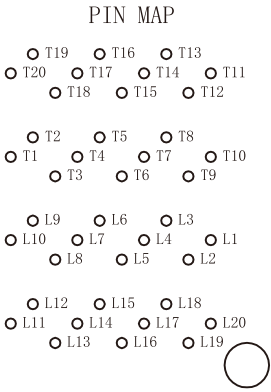
DETAIL D
