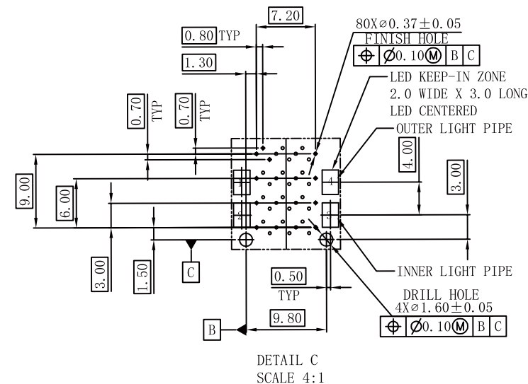
PIN MAP
