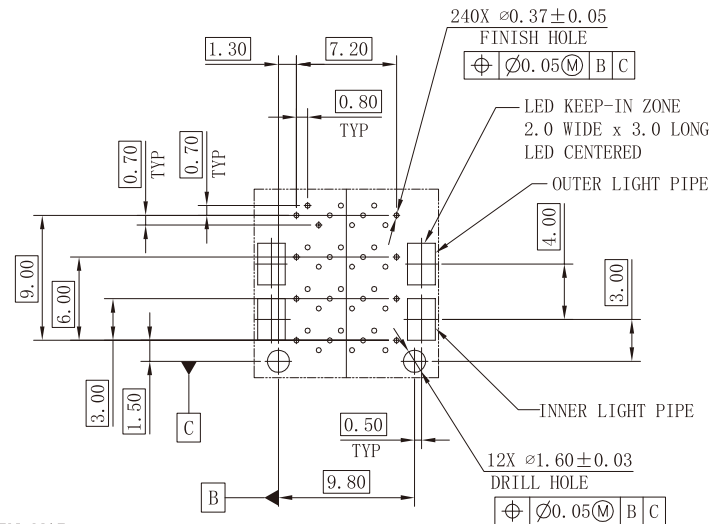
PIN MAP
