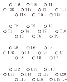
PIN MAP
