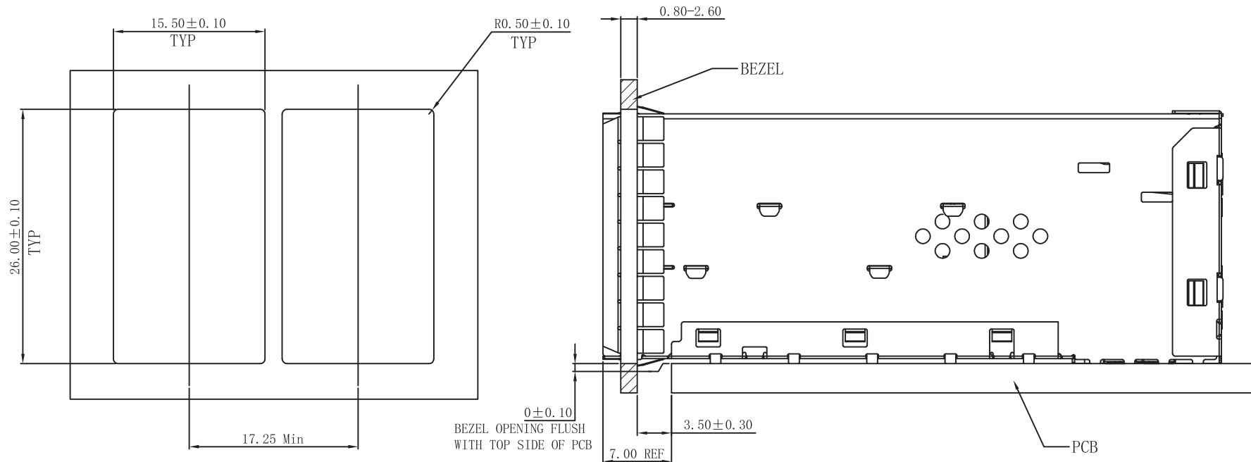
BEZEL CUT-OUT CENTER SPACING DETAIL BEZEL THICKNESS: 0.8-2.6
