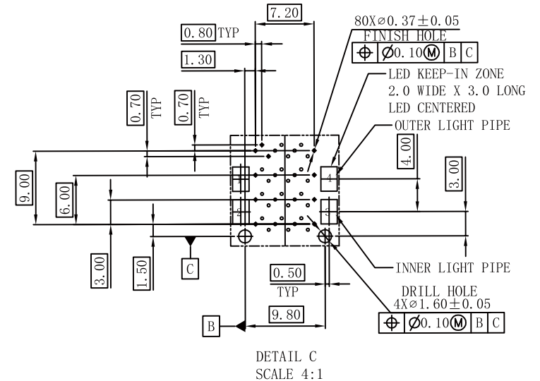
PIN MAP
