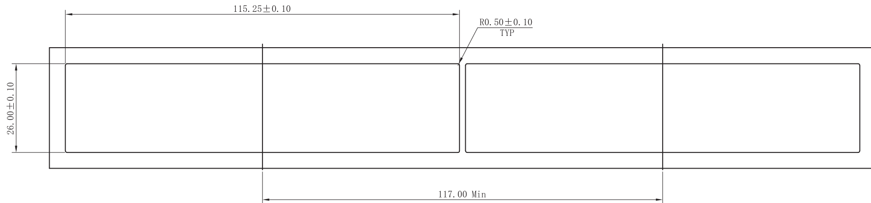
BEZEL CUT-OUT CENTER SPACING DETAIL BEZEL THICKNESS:0.8-2.6
