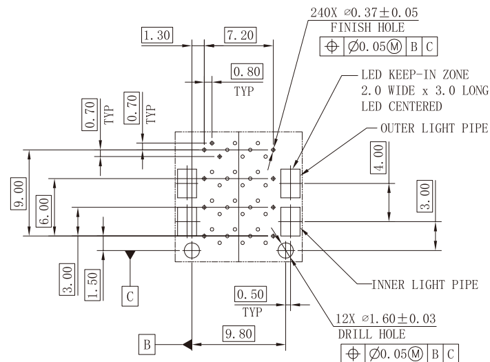
PIN MAP
