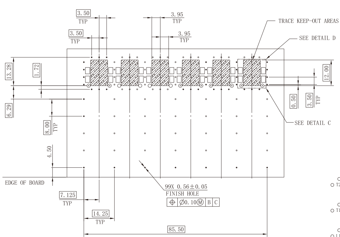
PIN MAP
