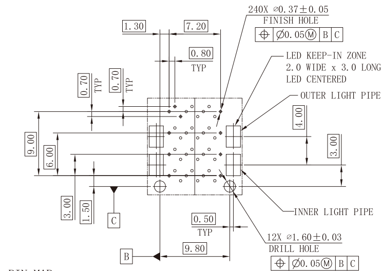
PIN MAP
