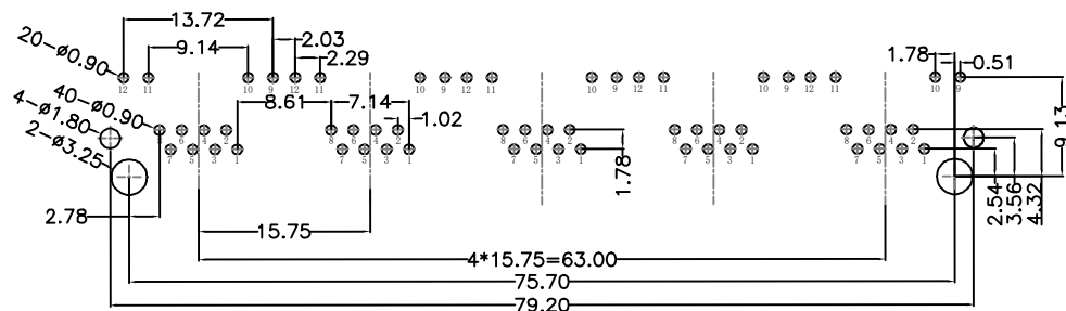
RECOMMENDED PCB LAYOUT VIEWED FROM COMPONENT SIDE
