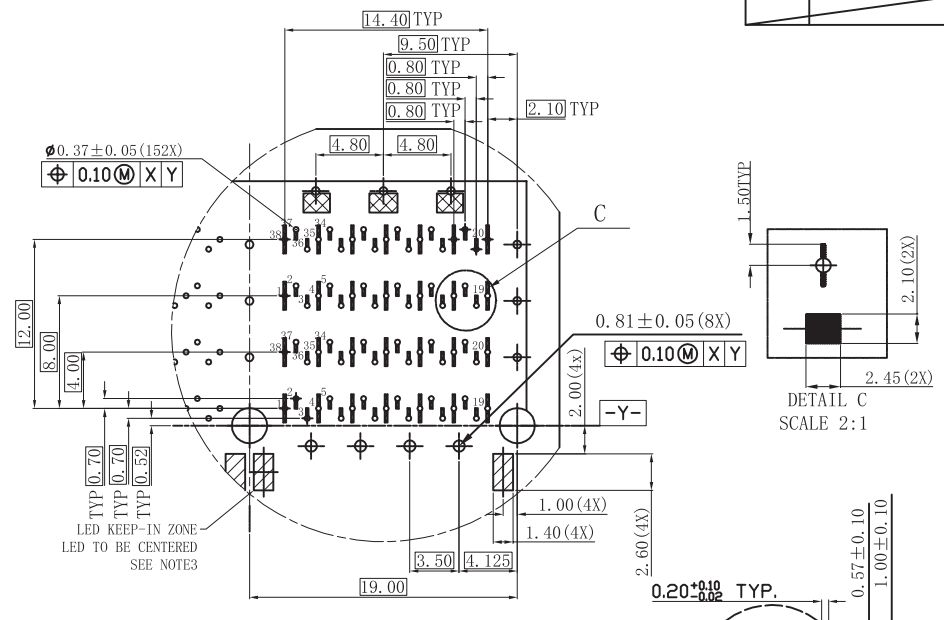
DETAIL B SCALE 2:1 PCB TOLERANCES ± 0.05 PCB PORT LAYOUT COMPONENT PORT
