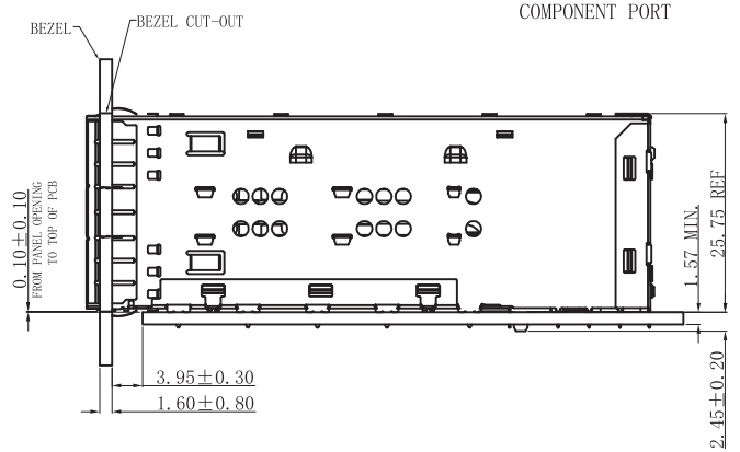
DETAIL B SCALE 2:1 PCB TOLERANCES ± 0.05 PCB PORT LAYOUT COMPONENT PORT
