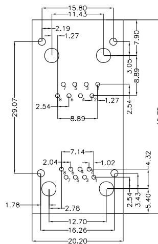
RECOMMENDED PCB LAYOUT VIEWED FROM COMPONENT SIDE
