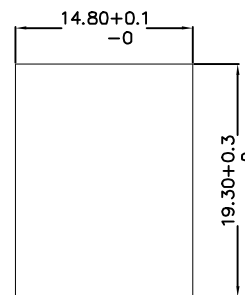
Single Panel-Latch Clearance Panel Thickness 1.60mm
