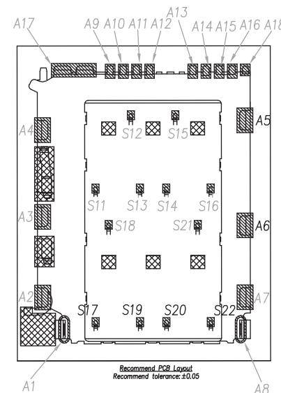
NANO SIM Block Pin Definition
