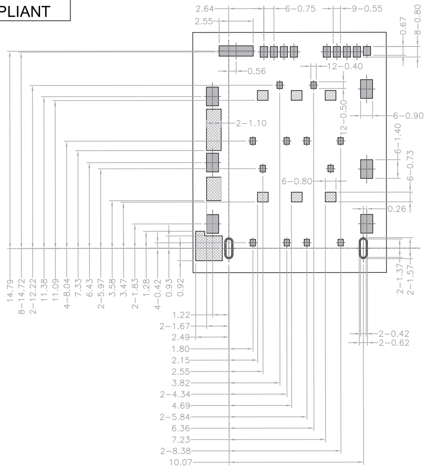
RECOMMENDED PCB LAYOUT(TOP VIEW) GENERAL TOLERANCE: \pm 0.05
